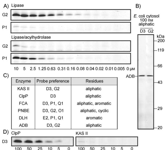
Figure 3. Sensitivity and specificity of the \beta -lactone library for individual enzymes. A) Concentration series of selected probes in the L. welshimeri proteome. B) ADB is the only enzyme in E. coli cytosol which is labeled by D3 and G2 at 100 nM. C) List of selected enzymes with their corresponding \beta -lactone probe preferences. D) In vivo labeling of L. welshimeri with \beta -lactone D3 at various concentrations.
