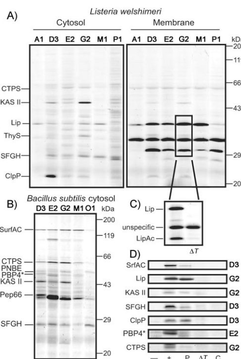
Figure 2. Labeling profiles of the \beta -lactone library against bacterial proteomes. A) Fluorescent gel of L. welshimeri cytosol and membrane proteomes after treatment with selected library members. The enzyme identities are assigned to the corresponding gel band (for a list of abbreviations, see Table 1). B) Fluorescent gel of B. subtilis cytosol proteome showing the identified enzyme targets. C) All reactions were carried out with a heat control ( \Delta T ) to identify unspecific labeling. An example is shown for G2 in the membrane proteome of L. welshimeri (boxed). D) Examples of recombinantly expressed enzymes (–: before induction, +: after induction, P: native proteome, \Delta T : after induction/heat control, C: after induction/no probe).
