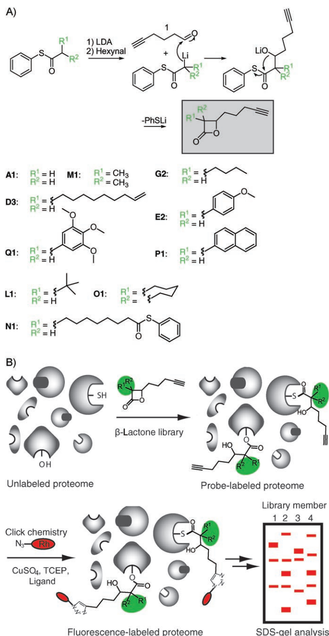
Figure 1. \beta -Lactones as privileged structures for bacterial ABPP. A) Synthetic route and biomimetic structures of the \beta -lactone library. LDA = lithium diisopropylamide B) Proteomes are first treated with the \beta -lactone library and subsequently appended with a fluorescent dye by click chemistry. Labeled proteomes were separated on sodium dodecyl sulfate polyacrylamide gel electrophoresis (SDS-PAGE) and visualized by fluorescence scanning.
